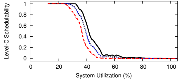
Figure 60: WSS 192.0, SRT, Way-First, Level-B Scaling Factor 3, Level-B tasks' Level-B utilization range [0.1,0.4], Level-C tasks' Level-C utilization range [0.5,0.9]
