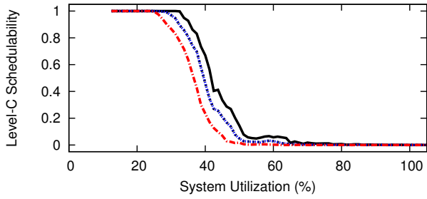
Figure 72: WSS 192.0, SRT, Way-First, Level-B Scaling Factor 5, Level-B tasks' Level-B utilization range [0.1,0.4], Level-C tasks' Level-C utilization range [0.5,0.9]
