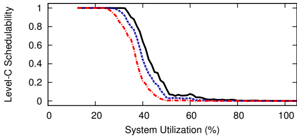
Figure 98: WSS 384.0, SRT, Color-First, Level-B Scaling Factor 5, Level-B tasks' Level-B utilization range [0.1,0.4], Level-C tasks' Level-C utilization range [0.5,0.9]
