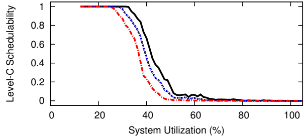
Figure 84: WSS 192.0, SRT, Color-First, Level-B Scaling Factor 3, Level-B tasks' Level-B utilization range [0.1,0.4], Level-C tasks' Level-C utilization range [0.5,0.9]
