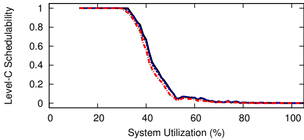
Figure 90: WSS 192.0, SRT, Color-First, Level-B Scaling Factor 5, Level-B tasks' Level-B utilization range [0.5,0.9], Level-C tasks' Level-C utilization range [0.5,0.9]
