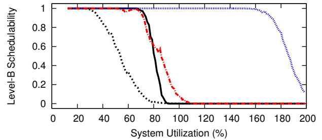
Figure 21: WSS 384.0, HRT, Way-First, Level-B Scaling Factor 5, Level-B tasks' Level-B utilization range [0.5,0.9], Level-C tasks' Level-C utilization range [0.5,0.9]
