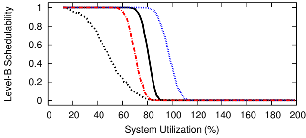
Figure 48: WSS 384.0, HRT, Color-First, Level-B Scaling Factor 5, Level-B tasks' Level-B utilization range [0.5,0.9], Level-C tasks' Level-C utilization range [0.1,0.4]
