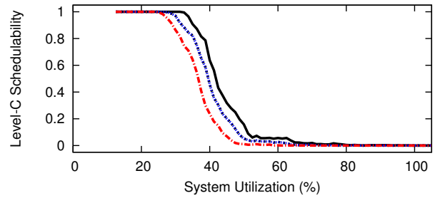
Figure 61: WSS 256.0, SRT, Way-First, Level-B Scaling Factor 3, Level-B tasks' Level-B utilization range [0.1,0.4], Level-C tasks' Level-C utilization range [0.5,0.9]
