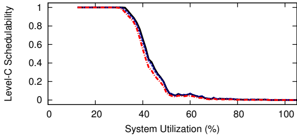
Figure 91: WSS 256.0, SRT, Color-First, Level-B Scaling Factor 5, Level-B tasks' Level-B utilization range [0.5,0.9], Level-C tasks' Level-C utilization range [0.5,0.9]
