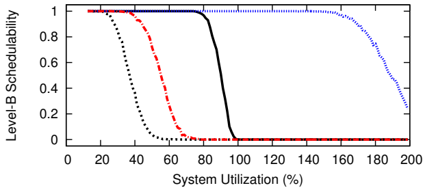
Figure 25: WSS 192.0, HRT, Way-First, Level-B Scaling Factor 5, Level-B tasks' Level-B utilization range [0.1,0.4], Level-C tasks' Level-C utilization range [0.5,0.9]
