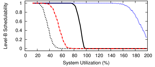
Figure 28: WSS 192.0, HRT, Way-First, Level-B Scaling Factor 5, Level-B tasks' Level-B utilization range [0.1,0.4], Level-C tasks' Level-C utilization range [0.1,0.4]
