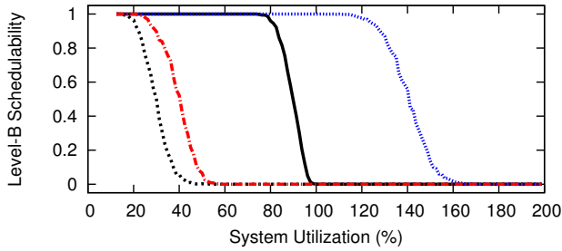
Figure 16: WSS 192.0, HRT, Way-First, Level-B Scaling Factor 3, Level-B tasks' Level-B utilization range [0.1,0.4], Level-C tasks' Level-C utilization range [0.1,0.4]
