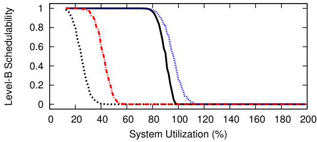
Figure 17: WSS 256.0, HRT, Way-First, Level-B Scaling Factor 3, Level-B tasks' Level-B utilization range [0.1,0.4], Level-C tasks' Level-C utilization range [0.1,0.4]
