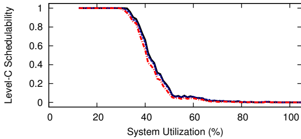
Figure 66: WSS 192.0, SRT, Way-First, Level-B Scaling Factor 5, Level-B tasks' Level-B utilization range [0.5,0.9], Level-C tasks' Level-C utilization range [0.5,0.9]
