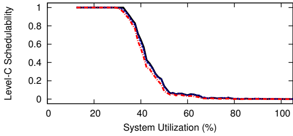
Figure 56: WSS 384.0, SRT, Way-First, Level-B Scaling Factor 3, Level-B tasks' Level-B utilization range [0.5,0.9], Level-C tasks' Level-C utilization range [0.5,0.9]
