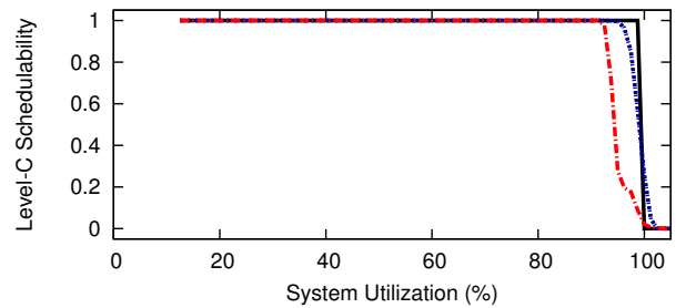
Figure 95: WSS 384.0, SRT, Color-First, Level-B Scaling Factor 5, Level-B tasks' Level-B utilization range [0.5,0.9], Level-C tasks' Level-C utilization range [0.1,0.4]
