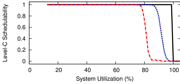
Figure 64: WSS 256.0, SRT, Way-First, Level-B Scaling Factor 3, Level-B tasks' Level-B utilization range [0.1,0.4], Level-C tasks' Level-C utilization range [0.1,0.4]
