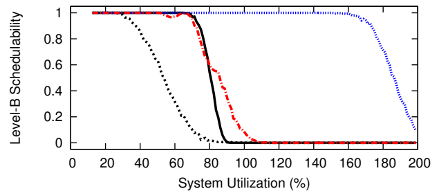
Figure 23: WSS 256.0, HRT, Way-First, Level-B Scaling Factor 5, Level-B tasks' Level-B utilization range [0.5,0.9], Level-C tasks' Level-C utilization range [0.1,0.4]
