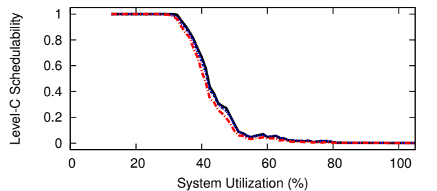
Figure 55: WSS 256.0, SRT, Way-First, Level-B Scaling Factor 3, Level-B tasks' Level-B utilization range [0.5,0.9], Level-C tasks' Level-C utilization range [0.5,0.9]
