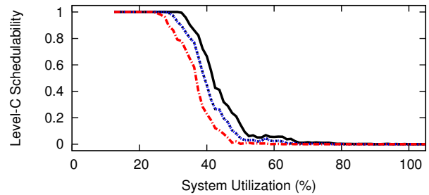
Figure 62: WSS 384.0, SRT, Way-First, Level-B Scaling Factor 3, Level-B tasks' Level-B utilization range [0.1,0.4], Level-C tasks' Level-C utilization range [0.5,0.9]
