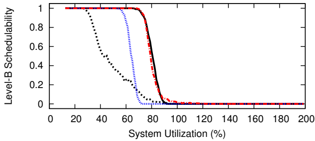
Figure 34: WSS 192.0, HRT, Color-First, Level-B Scaling Factor 3, Level-B tasks' Level-B utilization range [0.5,0.9], Level-C tasks' Level-C utilization range [0.1,0.4]
