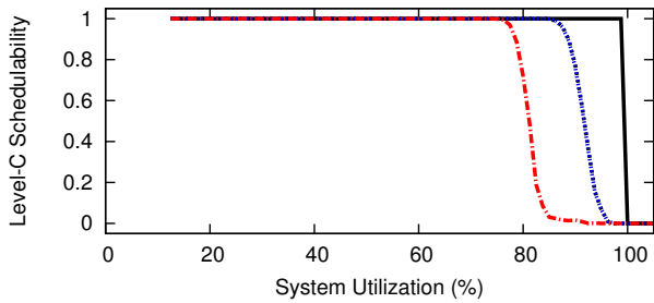
Figure 75: WSS 192.0, SRT, Way-First, Level-B Scaling Factor 5, Level-B tasks' Level-B utilization range [0.1,0.4], Level-C tasks' Level-C utilization range [0.1,0.4]
