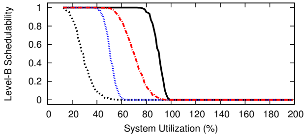
Figure 40: WSS 192.0, HRT, Color-First, Level-B Scaling Factor 3, Level-B tasks' Level-B utilization range [0.1,0.4], Level-C tasks' Level-C utilization range [0.1,0.4]
