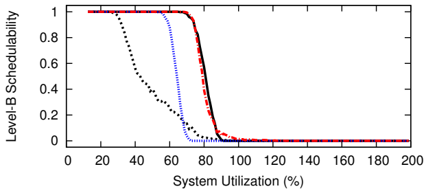
Figure 35: WSS 256.0, HRT, Color-First, Level-B Scaling Factor 3, Level-B tasks' Level-B utilization range [0.5,0.9], Level-C tasks' Level-C utilization range [0.1,0.4]
