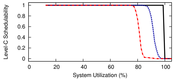
Figure 87: WSS 192.0, SRT, Color-First, Level-B Scaling Factor 3, Level-B tasks' Level-B utilization range [0.1,0.4], Level-C tasks' Level-C utilization range [0.1,0.4]
