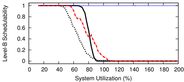
Figure 19: WSS 192.0, HRT, Way-First, Level-B Scaling Factor 5, Level-B tasks' Level-B utilization range [0.5,0.9], Level-C tasks' Level-C utilization range [0.5,0.9]
