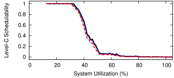
Figure 92: WSS 384.0, SRT, Color-First, Level-B Scaling Factor 5, Level-B tasks' Level-B utilization range [0.5,0.9], Level-C tasks' Level-C utilization range [0.5,0.9]
