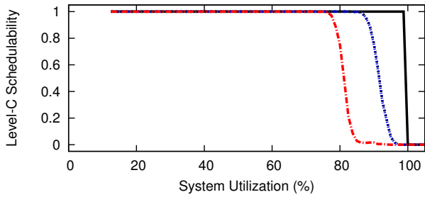
Figure 89: WSS 384.0, SRT, Color-First, Level-B Scaling Factor 3, Level-B tasks' Level-B utilization range [0.1,0.4], Level-C tasks' Level-C utilization range [0.1,0.4]
