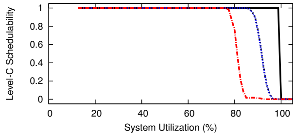
Figure 77: WSS 384.0, SRT, Way-First, Level-B Scaling Factor 5, Level-B tasks' Level-B utilization range [0.1,0.4], Level-C tasks' Level-C utilization range [0.1,0.4]
