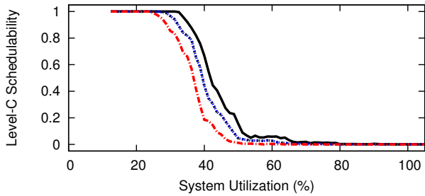
Figure 74: WSS 384.0, SRT, Way-First, Level-B Scaling Factor 5, Level-B tasks' Level-B utilization range [0.1,0.4], Level-C tasks' Level-C utilization range [0.5,0.9]
