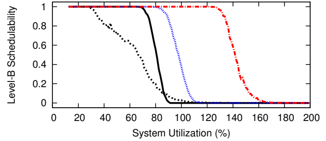
Figure 44: WSS 256.0, HRT, Color-First, Level-B Scaling Factor 5, Level-B tasks' Level-B utilization range [0.5,0.9], Level-C tasks' Level-C utilization range [0.5,0.9]
