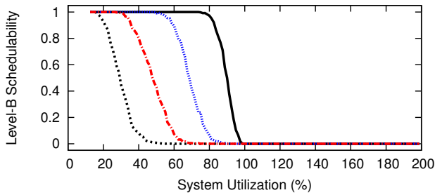
Figure 51: WSS 384.0, HRT, Color-First, Level-B Scaling Factor 5, Level-B tasks' Level-B utilization range [0.1,0.4], Level-C tasks' Level-C utilization range [0.5,0.9]
