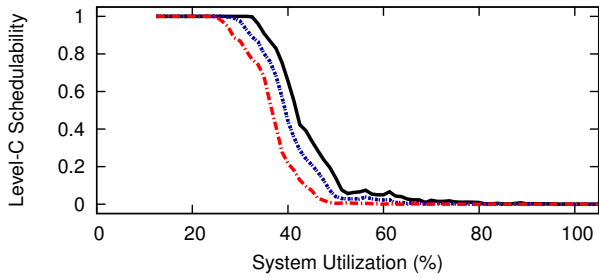
Figure 97: WSS 256.0, SRT, Color-First, Level-B Scaling Factor 5, Level-B tasks' Level-B utilization range [0.1,0.4], Level-C tasks' Level-C utilization range [0.5,0.9]
