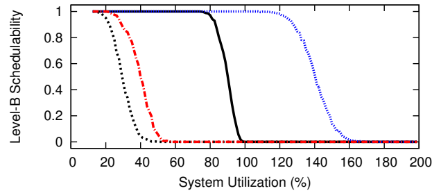
Figure 13: WSS 192.0, HRT, Way-First, Level-B Scaling Factor 3, Level-B tasks' Level-B utilization range [0.1,0.4], Level-C tasks' Level-C utilization range [0.5,0.9]
