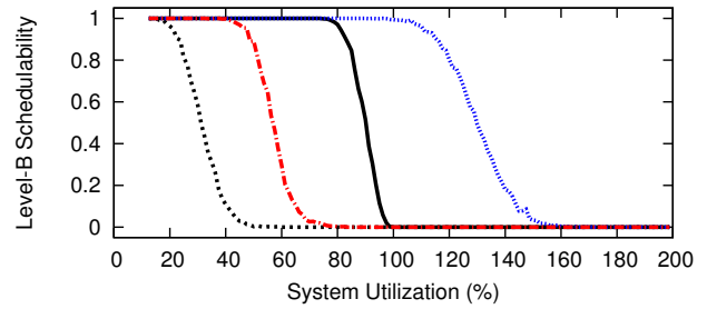
Figure 29: WSS 256.0, HRT, Way-First, Level-B Scaling Factor 5, Level-B tasks' Level-B utilization range [0.1,0.4], Level-C tasks' Level-C utilization range [0.1,0.4]
