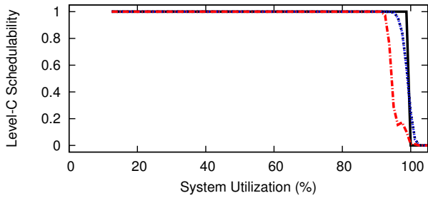
Figure 57: WSS 192.0, SRT, Way-First, Level-B Scaling Factor 3, Level-B tasks' Level-B utilization range [0.5,0.9], Level-C tasks' Level-C utilization range [0.1,0.4]
