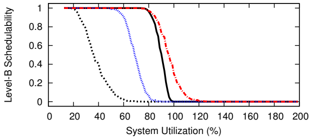
Figure 50: WSS 256.0, HRT, Color-First, Level-B Scaling Factor 5, Level-B tasks' Level-B utilization range [0.1,0.4], Level-C tasks' Level-C utilization range [0.5,0.9]
