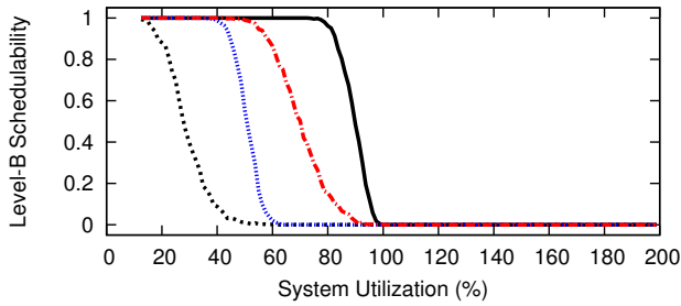
Figure 41: WSS 256.0, HRT, Color-First, Level-B Scaling Factor 3, Level-B tasks' Level-B utilization range [0.1,0.4], Level-C tasks' Level-C utilization range [0.1,0.4]
