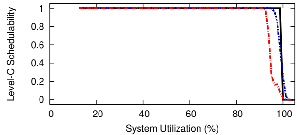
Figure 94: WSS 256.0, SRT, Color-First, Level-B Scaling Factor 5, Level-B tasks' Level-B utilization range [0.5,0.9], Level-C tasks' Level-C utilization range [0.1,0.4]
