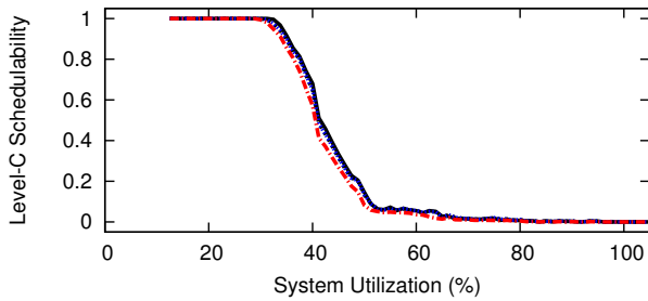
Figure 67: WSS 256.0, SRT, Way-First, Level-B Scaling Factor 5, Level-B tasks' Level-B utilization range [0.5,0.9], Level-C tasks' Level-C utilization range [0.5,0.9]
