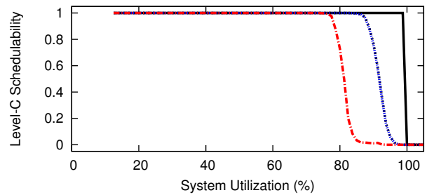
Figure 63: WSS 192.0, SRT, Way-First, Level-B Scaling Factor 3, Level-B tasks' Level-B utilization range [0.1,0.4], Level-C tasks' Level-C utilization range [0.1,0.4]
