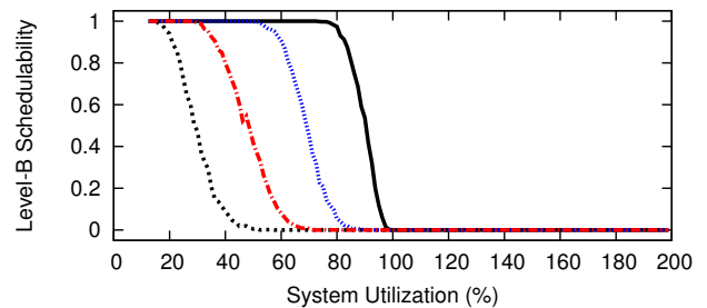
Figure 54: WSS 384.0, HRT, Color-First, Level-B Scaling Factor 5, Level-B tasks' Level-B utilization range [0.1,0.4], Level-C tasks' Level-C utilization range [0.1,0.4]
