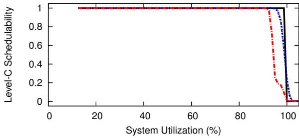
Figure 81: WSS 192.0, SRT, Color-First, Level-B Scaling Factor 3, Level-B tasks' Level-B utilization range [0.5,0.9], Level-C tasks' Level-C utilization range [0.1,0.4]
