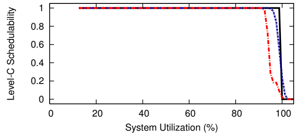
Figure 93: WSS 192.0, SRT, Color-First, Level-B Scaling Factor 5, Level-B tasks' Level-B utilization range [0.5,0.9], Level-C tasks' Level-C utilization range [0.1,0.4]
