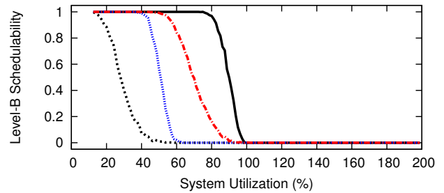
Figure 38: WSS 256.0, HRT, Color-First, Level-B Scaling Factor 3, Level-B tasks' Level-B utilization range [0.1,0.4], Level-C tasks' Level-C utilization range [0.5,0.9]
