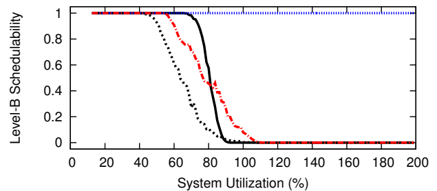
Figure 22: WSS 192.0, HRT, Way-First, Level-B Scaling Factor 5, Level-B tasks' Level-B utilization range [0.5,0.9], Level-C tasks' Level-C utilization range [0.1,0.4]
