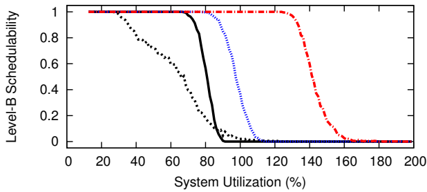
Figure 43: WSS 192.0, HRT, Color-First, Level-B Scaling Factor 5, Level-B tasks' Level-B utilization range [0.5,0.9], Level-C tasks' Level-C utilization range [0.5,0.9]
