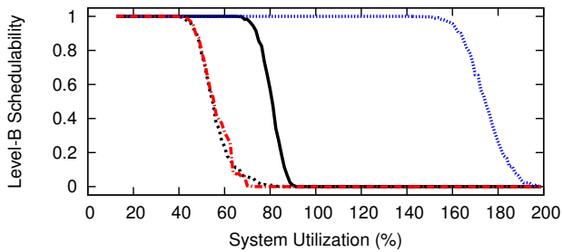
Figure 10: WSS 192.0, HRT, Way-First, Level-B Scaling Factor 3, Level-B tasks' Level-B utilization range [0.5,0.9], Level-C tasks' Level-C utilization range [0.1,0.4]
