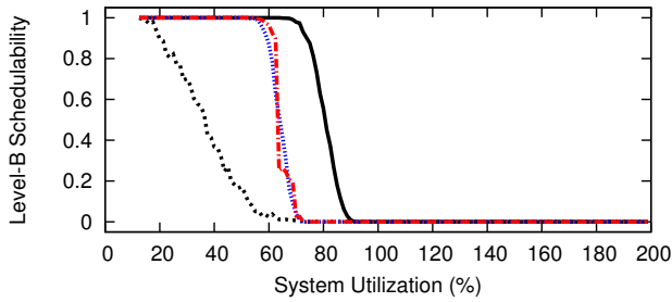
Figure 33: WSS 384.0, HRT, Color-First, Level-B Scaling Factor 3, Level-B tasks' Level-B utilization range [0.5,0.9], Level-C tasks' Level-C utilization range [0.5,0.9]
