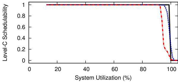
Figure 58: WSS 256.0, SRT, Way-First, Level-B Scaling Factor 3, Level-B tasks' Level-B utilization range [0.5,0.9], Level-C tasks' Level-C utilization range [0.1,0.4]
