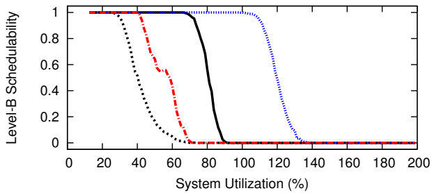
Figure 11: WSS 256.0, HRT, Way-First, Level-B Scaling Factor 3, Level-B tasks' Level-B utilization range [0.5,0.9], Level-C tasks' Level-C utilization range [0.1,0.4]
