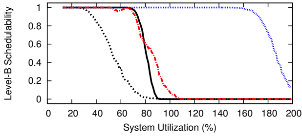
Figure 24: WSS 384.0, HRT, Way-First, Level-B Scaling Factor 5, Level-B tasks' Level-B utilization range [0.5,0.9], Level-C tasks' Level-C utilization range [0.1,0.4]
