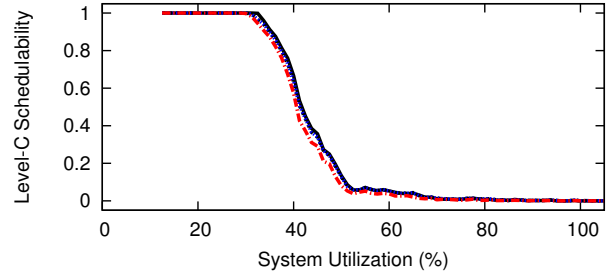
Figure 68: WSS 384.0, SRT, Way-First, Level-B Scaling Factor 5, Level-B tasks' Level-B utilization range [0.5,0.9], Level-C tasks' Level-C utilization range [0.5,0.9]
