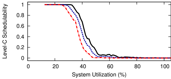
Figure 73: WSS 256.0, SRT, Way-First, Level-B Scaling Factor 5, Level-B tasks' Level-B utilization range [0.1,0.4], Level-C tasks' Level-C utilization range [0.5,0.9]
