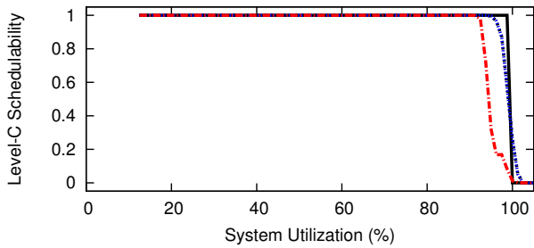
Figure 59: WSS 384.0, SRT, Way-First, Level-B Scaling Factor 3, Level-B tasks' Level-B utilization range [0.5,0.9], Level-C tasks' Level-C utilization range [0.1,0.4]
