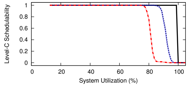
Figure 101: WSS 384.0, SRT, Color-First, Level-B Scaling Factor 5, Level-B tasks' Level-B utilization range [0.1,0.4], Level-C tasks' Level-C utilization range [0.1,0.4]
