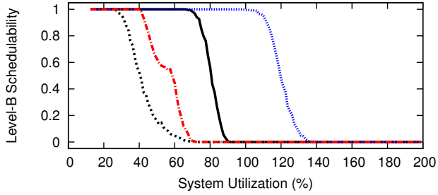
Figure 9: WSS 384.0, HRT, Way-First, Level-B Scaling Factor 3, Level-B tasks' Level-B utilization range [0.5,0.9], Level-C tasks' Level-C utilization range [0.5,0.9]
