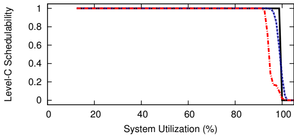
Figure 83: WSS 384.0, SRT, Color-First, Level-B Scaling Factor 3, Level-B tasks' Level-B utilization range [0.5,0.9], Level-C tasks' Level-C utilization range [0.1,0.4]
