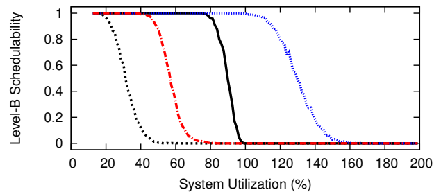
Figure 30: WSS 384.0, HRT, Way-First, Level-B Scaling Factor 5, Level-B tasks' Level-B utilization range [0.1,0.4], Level-C tasks' Level-C utilization range [0.1,0.4]
