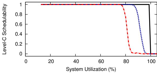
Figure 99: WSS 192.0, SRT, Color-First, Level-B Scaling Factor 5, Level-B tasks' Level-B utilization range [0.1,0.4], Level-C tasks' Level-C utilization range [0.1,0.4]
