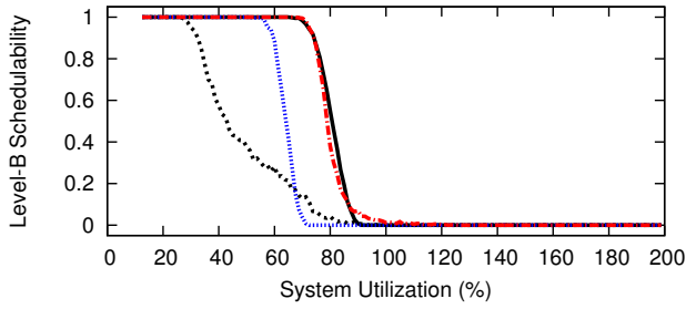
Figure 32: WSS 256.0, HRT, Color-First, Level-B Scaling Factor 3, Level-B tasks' Level-B utilization range [0.5,0.9], Level-C tasks' Level-C utilization range [0.5,0.9]
