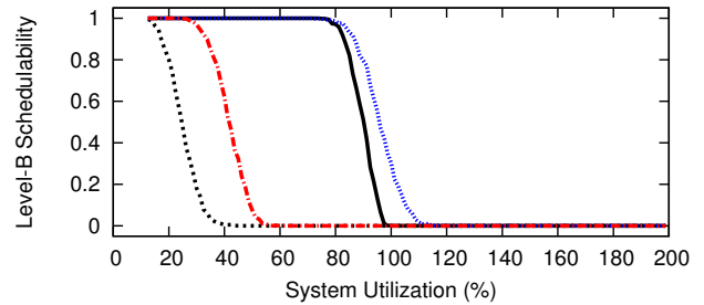
Figure 15: WSS 384.0, HRT, Way-First, Level-B Scaling Factor 3, Level-B tasks' Level-B utilization range [0.1,0.4], Level-C tasks' Level-C utilization range [0.5,0.9]
