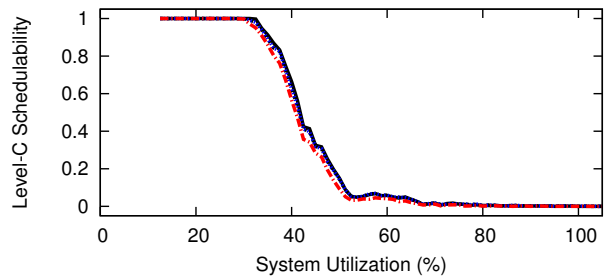
Figure 79: WSS 256.0, SRT, Color-First, Level-B Scaling Factor 3, Level-B tasks' Level-B utilization range [0.5,0.9], Level-C tasks' Level-C utilization range [0.5,0.9]
