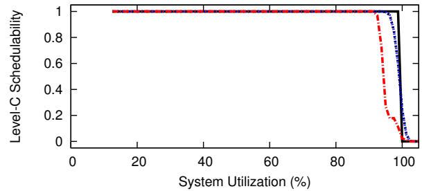
Figure 69: WSS 192.0, SRT, Way-First, Level-B Scaling Factor 5, Level-B tasks' Level-B utilization range [0.5,0.9], Level-C tasks' Level-C utilization range [0.1,0.4]
