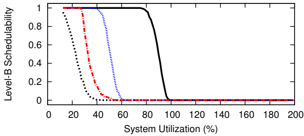
Figure 42: WSS 384.0, HRT, Color-First, Level-B Scaling Factor 3, Level-B tasks' Level-B utilization range [0.1,0.4], Level-C tasks' Level-C utilization range [0.1,0.4]
