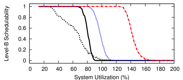
Figure 47: WSS 256.0, HRT, Color-First, Level-B Scaling Factor 5, Level-B tasks' Level-B utilization range [0.5,0.9], Level-C tasks' Level-C utilization range [0.1,0.4]
