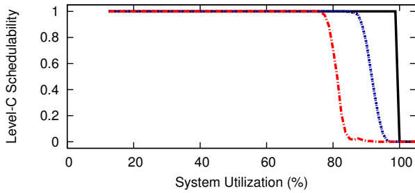
Figure 65: WSS 384.0, SRT, Way-First, Level-B Scaling Factor 3, Level-B tasks' Level-B utilization range [0.1,0.4], Level-C tasks' Level-C utilization range [0.1,0.4]
