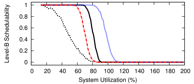
Figure 45: WSS 384.0, HRT, Color-First, Level-B Scaling Factor 5, Level-B tasks' Level-B utilization range [0.5,0.9], Level-C tasks' Level-C utilization range [0.5,0.9]
