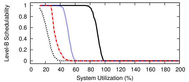
Figure 39: WSS 384.0, HRT, Color-First, Level-B Scaling Factor 3, Level-B tasks' Level-B utilization range [0.1,0.4], Level-C tasks' Level-C utilization range [0.5,0.9]
