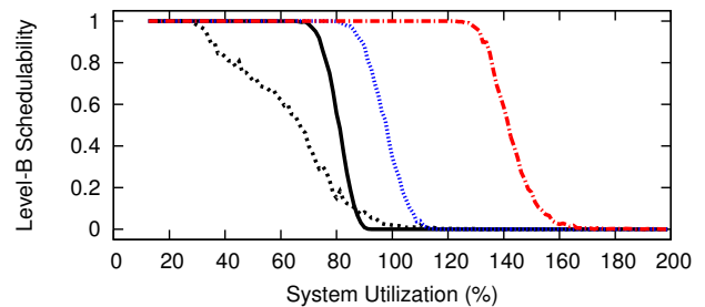
Figure 46: WSS 192.0, HRT, Color-First, Level-B Scaling Factor 5, Level-B tasks' Level-B utilization range [0.5,0.9], Level-C tasks' Level-C utilization range [0.1,0.4]
