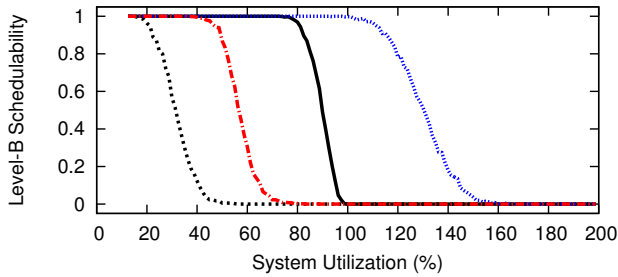
Figure 26: WSS 256.0, HRT, Way-First, Level-B Scaling Factor 5, Level-B tasks' Level-B utilization range [0.1,0.4], Level-C tasks' Level-C utilization range [0.5,0.9]
