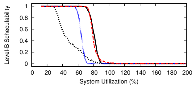
Figure 31: WSS 192.0, HRT, Color-First, Level-B Scaling Factor 3, Level-B tasks' Level-B utilization range [0.5,0.9], Level-C tasks' Level-C utilization range [0.5,0.9]
