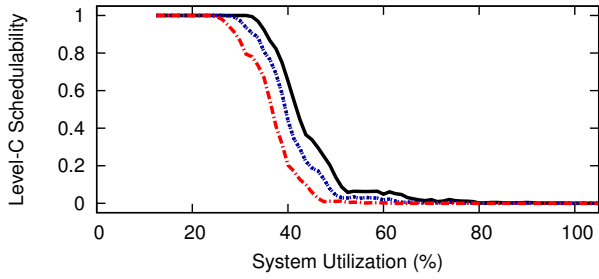
Figure 96: WSS 192.0, SRT, Color-First, Level-B Scaling Factor 5, Level-B tasks' Level-B utilization range [0.1,0.4], Level-C tasks' Level-C utilization range [0.5,0.9]
