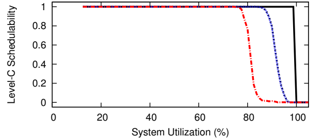
Figure 100: WSS 256.0, SRT, Color-First, Level-B Scaling Factor 5, Level-B tasks' Level-B utilization range [0.1,0.4], Level-C tasks' Level-C utilization range [0.1,0.4]
