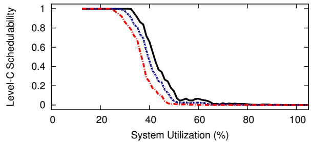
Figure 86: WSS 384.0, SRT, Color-First, Level-B Scaling Factor 3, Level-B tasks' Level-B utilization range [0.1,0.4], Level-C tasks' Level-C utilization range [0.5,0.9]
