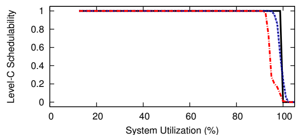
Figure 71: WSS 384.0, SRT, Way-First, Level-B Scaling Factor 5, Level-B tasks' Level-B utilization range [0.5,0.9], Level-C tasks' Level-C utilization range [0.1,0.4]
