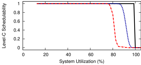
Figure 88: WSS 256.0, SRT, Color-First, Level-B Scaling Factor 3, Level-B tasks' Level-B utilization range [0.1,0.4], Level-C tasks' Level-C utilization range [0.1,0.4]
