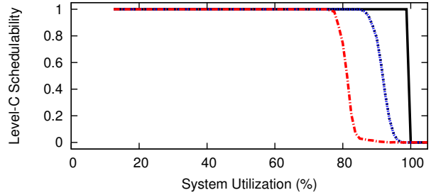
Figure 76: WSS 256.0, SRT, Way-First, Level-B Scaling Factor 5, Level-B tasks' Level-B utilization range [0.1,0.4], Level-C tasks' Level-C utilization range [0.1,0.4]
