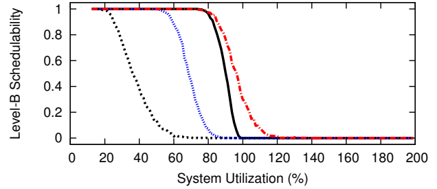
Figure 52: WSS 192.0, HRT, Color-First, Level-B Scaling Factor 5, Level-B tasks' Level-B utilization range [0.1,0.4], Level-C tasks' Level-C utilization range [0.1,0.4]
