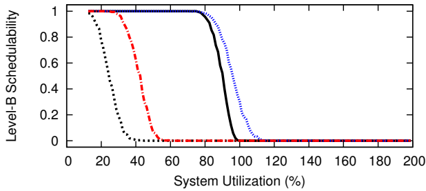
Figure 18: WSS 384.0, HRT, Way-First, Level-B Scaling Factor 3, Level-B tasks' Level-B utilization range [0.1,0.4], Level-C tasks' Level-C utilization range [0.1,0.4]
