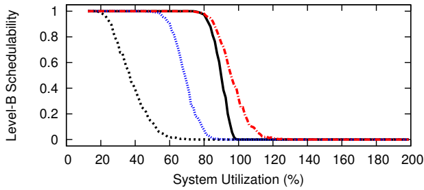
Figure 49: WSS 192.0, HRT, Color-First, Level-B Scaling Factor 5, Level-B tasks' Level-B utilization range [0.1,0.4], Level-C tasks' Level-C utilization range [0.5,0.9]
