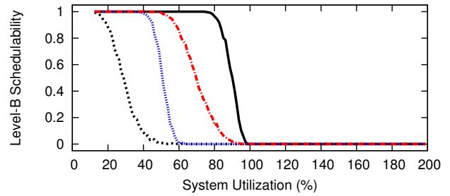
Figure 37: WSS 192.0, HRT, Color-First, Level-B Scaling Factor 3, Level-B tasks' Level-B utilization range [0.1,0.4], Level-C tasks' Level-C utilization range [0.5,0.9]
