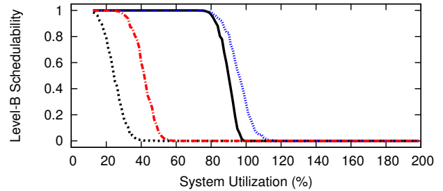
Figure 14: WSS 256.0, HRT, Way-First, Level-B Scaling Factor 3, Level-B tasks' Level-B utilization range [0.1,0.4], Level-C tasks' Level-C utilization range [0.5,0.9]
