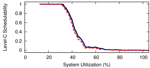
Figure 78: WSS 192.0, SRT, Color-First, Level-B Scaling Factor 3, Level-B tasks' Level-B utilization range [0.5,0.9], Level-C tasks' Level-C utilization range [0.5,0.9]
