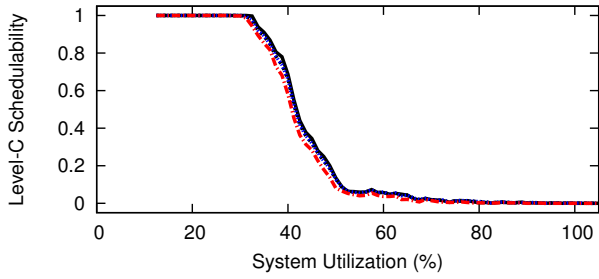
Figure 80: WSS 384.0, SRT, Color-First, Level-B Scaling Factor 3, Level-B tasks' Level-B utilization range [0.5,0.9], Level-C tasks' Level-C utilization range [0.5,0.9]
