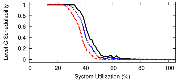
Figure 85: WSS 256.0, SRT, Color-First, Level-B Scaling Factor 3, Level-B tasks' Level-B utilization range [0.1,0.4], Level-C tasks' Level-C utilization range [0.5,0.9]
