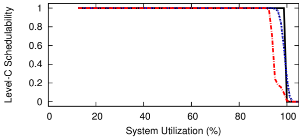
Figure 82: WSS 256.0, SRT, Color-First, Level-B Scaling Factor 3, Level-B tasks' Level-B utilization range [0.5,0.9], Level-C tasks' Level-C utilization range [0.1,0.4]
