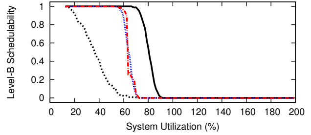
Figure 36: WSS 384.0, HRT, Color-First, Level-B Scaling Factor 3, Level-B tasks' Level-B utilization range [0.5,0.9], Level-C tasks' Level-C utilization range [0.1,0.4]
