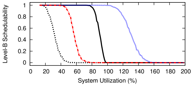
Figure 27: WSS 384.0, HRT, Way-First, Level-B Scaling Factor 5, Level-B tasks' Level-B utilization range [0.1,0.4], Level-C tasks' Level-C utilization range [0.5,0.9]
