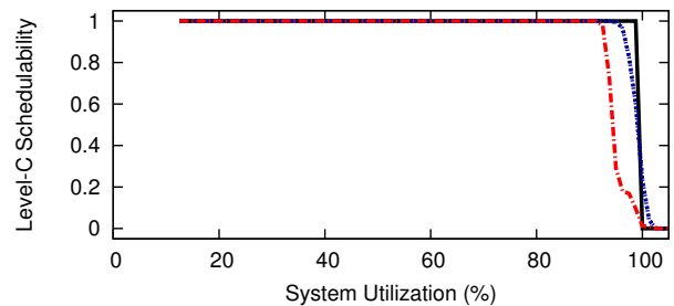
Figure 70: WSS 256.0, SRT, Way-First, Level-B Scaling Factor 5, Level-B tasks' Level-B utilization range [0.5,0.9], Level-C tasks' Level-C utilization range [0.1,0.4]
