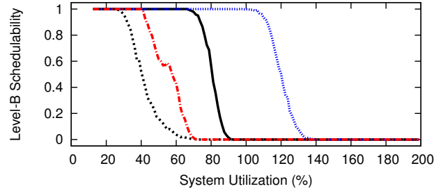
Figure 12: WSS 384.0, HRT, Way-First, Level-B Scaling Factor 3, Level-B tasks' Level-B utilization range [0.5,0.9], Level-C tasks' Level-C utilization range [0.1,0.4]
