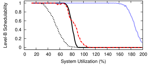
Figure 20: WSS 256.0, HRT, Way-First, Level-B Scaling Factor 5, Level-B tasks' Level-B utilization range [0.5,0.9], Level-C tasks' Level-C utilization range [0.5,0.9]
