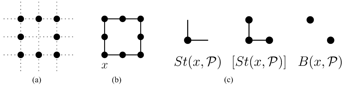
Fig. 5. Using the polyhedron approach to determine if a point x is simple. The loop case. Point x is not simple. (a) Set of points \mathcal{P} . (b) Polyhedron \Pi(\mathcal{P}) . (c) Determining the base B(x, \mathcal{P}) .
