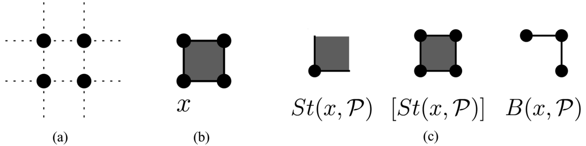
Fig. 6. Using the polyhedron approach to determine if a point x is simple. The square case. Point x is simple. (a) Set of points \mathcal{P} . (b) Polyhedron \Pi(\mathcal{P}) . (c) Determining the base B(x, \mathcal{P}) .
