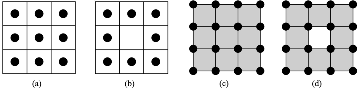
Fig. 4. Removing a pixel in a 2-D digital image. Illustration of the point and the unitary cube based approaches. (a) One point per pixel before removal of the center pixel. (b) One point per pixel after removal of the center pixel. (c) One unitary cube per pixel before removal of the center pixel. (d) One unitary cube per pixel after removal of the center pixel.
