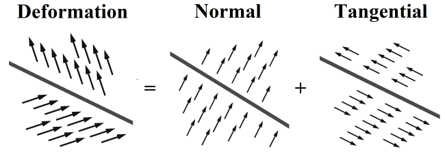
(a) Decomposition of the deformation field u into the motion normal to the organ boundary ( u^\perp ) and the motion tangential to the organ boundary ( u^\parallel ). The straight line represents the organ boundary.
