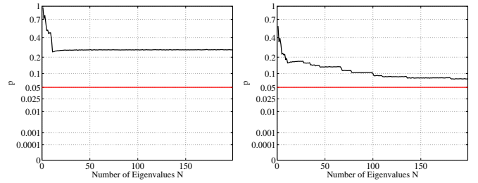
Fig. 26. Accumulative maximum t-statistic results (unit intracranial content, Dirichlet) for the regular (left) and the dual (right) voxel graphs. Employing the dual graph yields lower p -values. This may be attributed to the better suitability of the dual graph for probing the thin tail regions of the caudate shapes. However, there is no statistical difference at a significance level of \alpha = 5\% .
