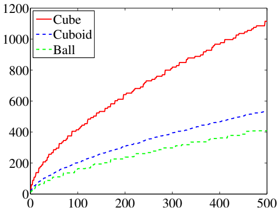
Fig. 5. Unnormalized exact spectra of cube, cuboid, ball.
