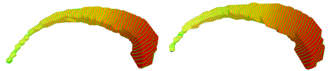
Fig. 22. 100 level sets wrapped around two exemplary caudate shapes using the first eigenfunction. The absence of any saddles guarantees that each level set has only one component.
