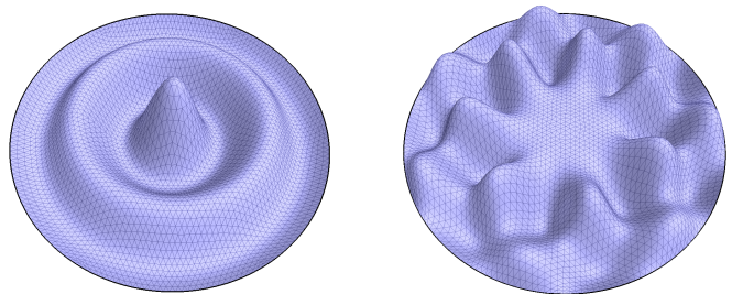
Fig. 1. Eigenfunction 30 and 50 of the disk.
