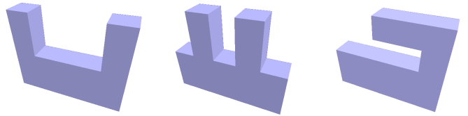
Fig. 2. Objects with same shape index but different spectra
