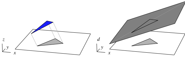
Figure 5: A polygonal primitive and its region of influence in a slice (left). The corresponding linear distance function (right).
